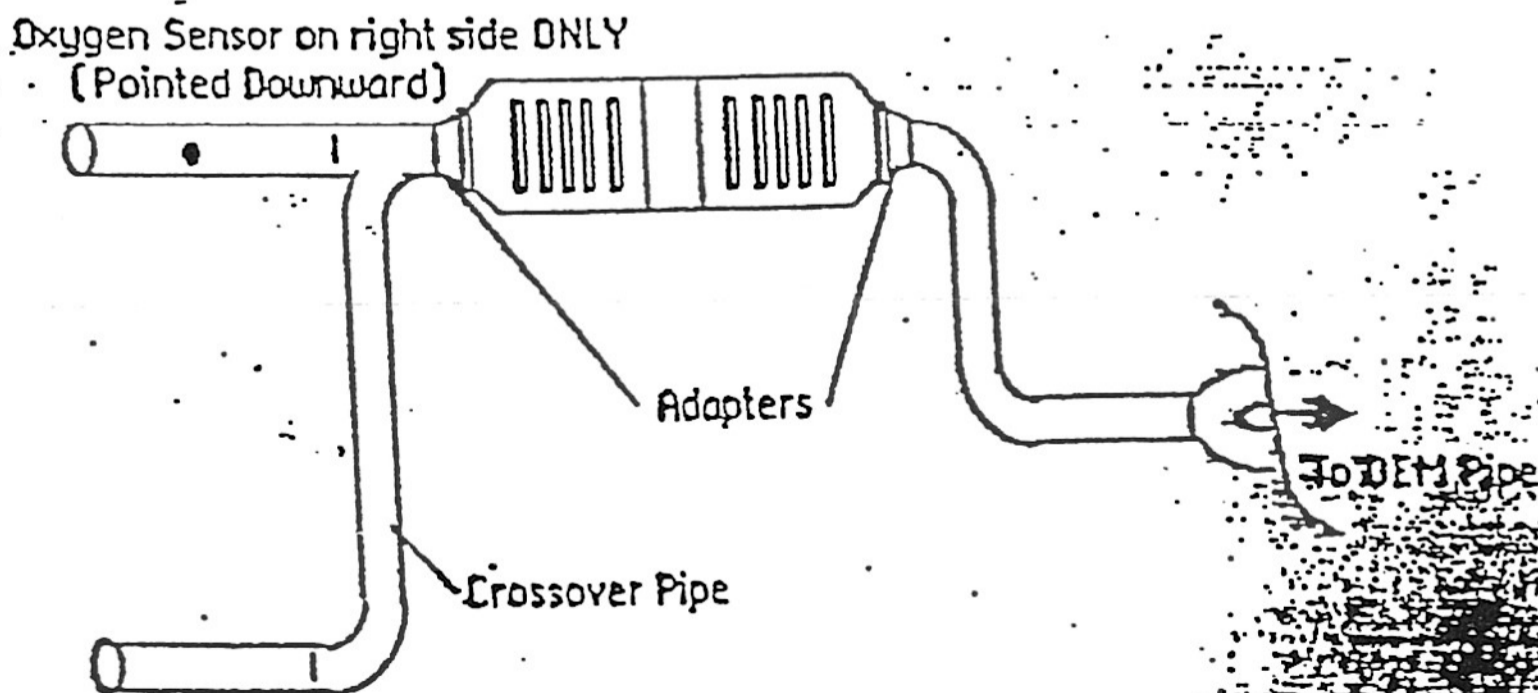
Side view of Catalytic Converter Layout [Not to scale] [Left side down pipe omitted for clarity]
